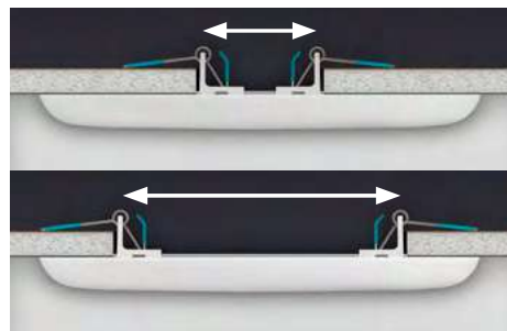
18.5W bracket adjusts from 65mm to 205mm
