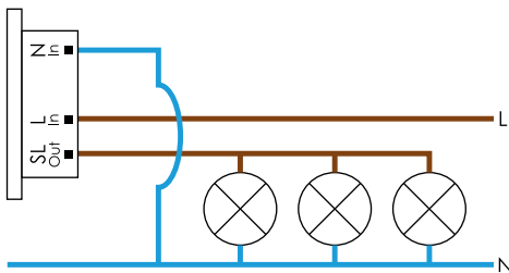
Wiring Diagram
