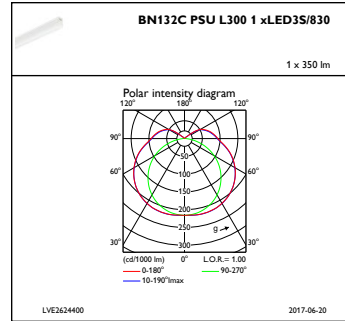
IFPC1_BN132CPSUL3001xLED3S830
